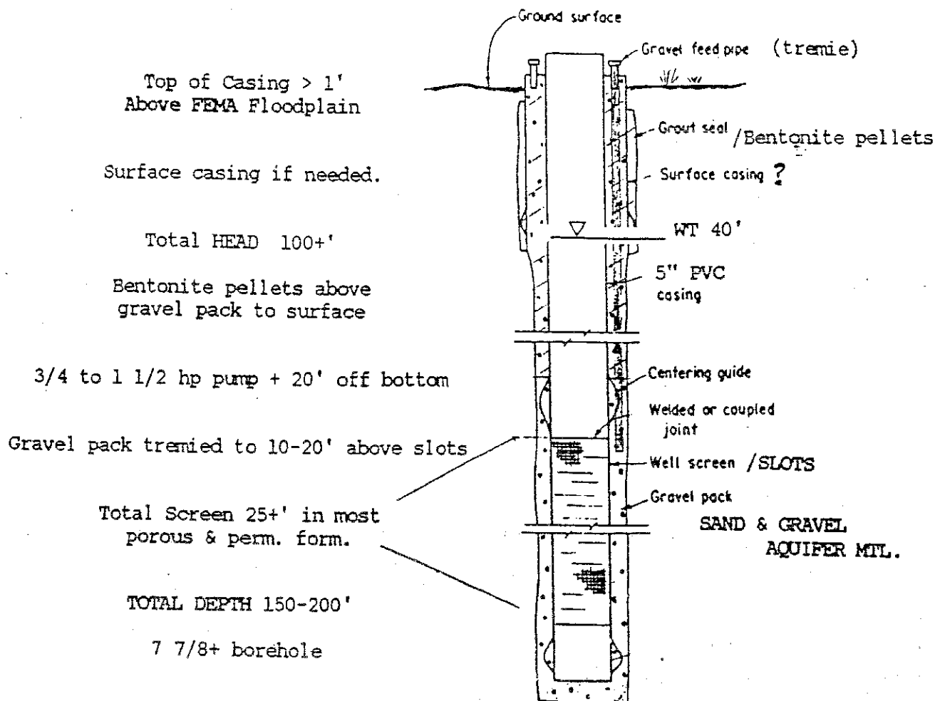
SINGLE STRING CONSTRUCTION
