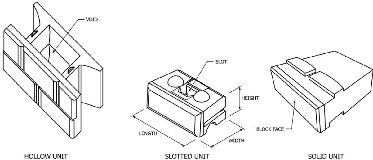
FIG. X1.1 Typical Examples of Precast Modular Retaining Wall Units
