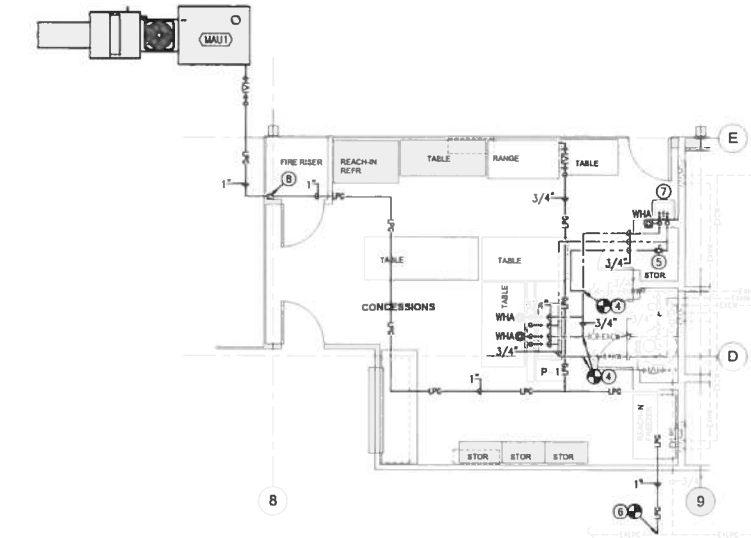
PLUMBING CONCESSION PLAN - DOMESTIC WATER AND GAS SCALE: 1/4" = 1'-0"
