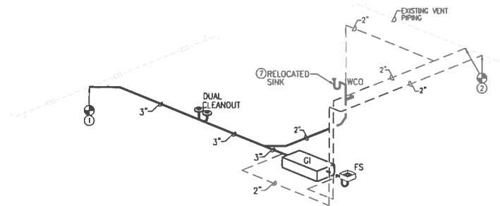
PLUMBING RISER DIAGRAM - SANITARY WASTE AND VENT SCALE: 1/4" = 1'-0"
