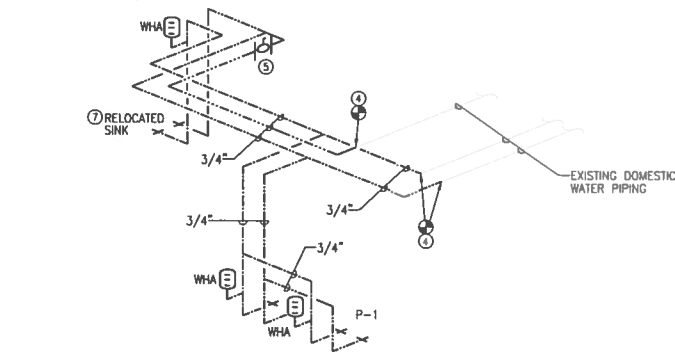
PLUMBING RISER DIAGRAM - DOMESTIC WATER AND GAS SCALE: 1/4" = 1'-0"
