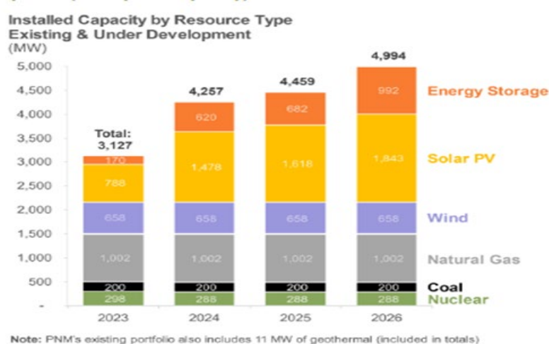
Figure 4: PNM's Current Generation Portfolio, including existing resources and resources under development (nameplate capacity) 2023-2026
