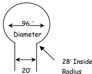
Cul-de-sac Turnaround
