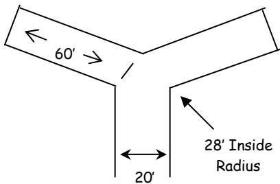
Typical Y-Turn Turnaround
