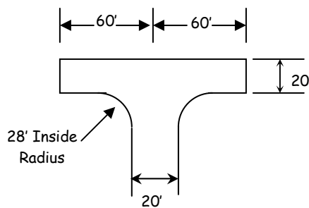
Typical Hammerhead Turnaround
