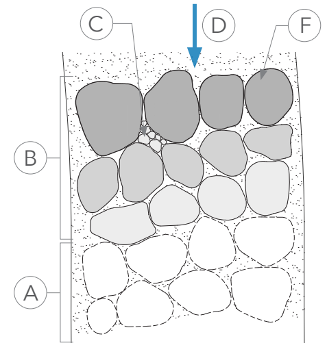
Plan Detail One Rock Dam
