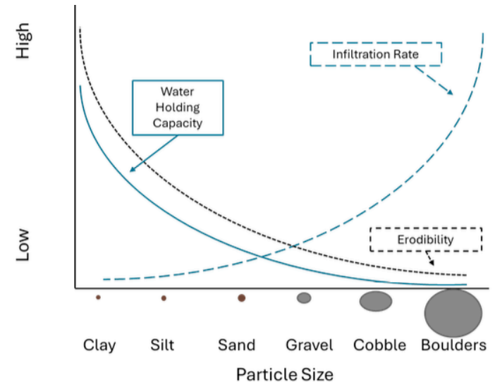
Chart illustrating the relationship between particle size, water holding capacity, and infiltrate rate.
