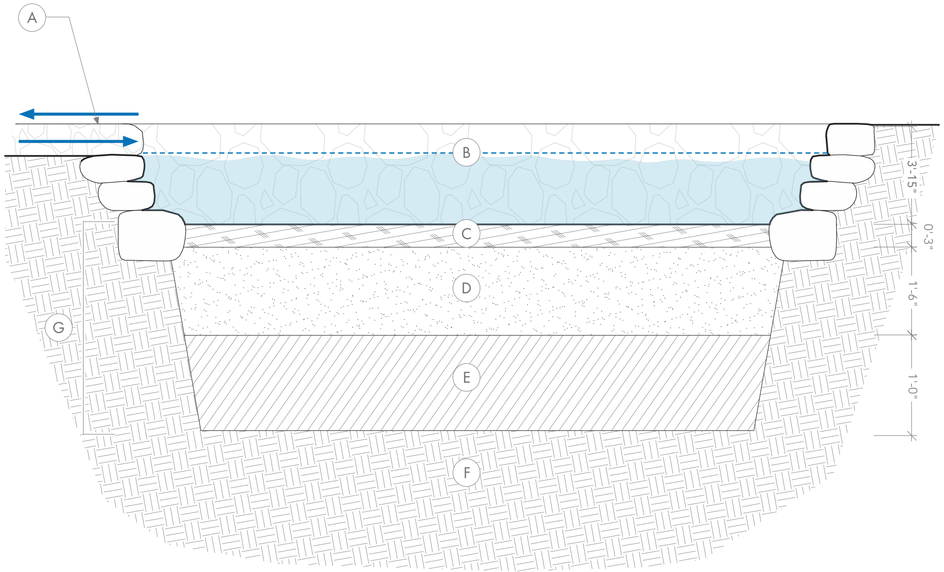
Cross Section of Bioretention Basin
