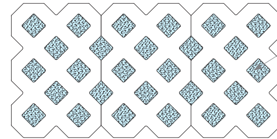
Plan detail of CGPs assembled in interlocking group
