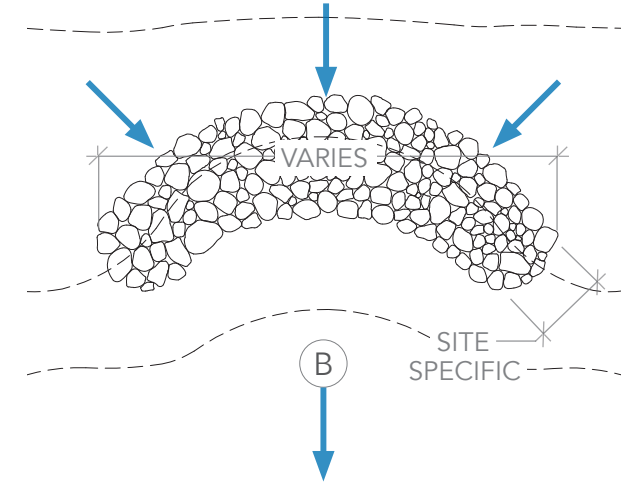
Plan Detail "Tips Down" Media Luna
