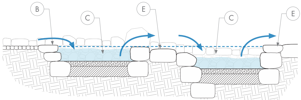
Urban Zuni Bowl Section
