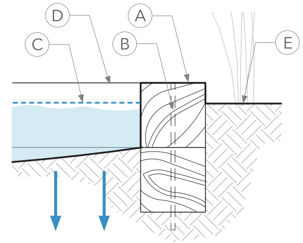
Wooden Basin Border Section
