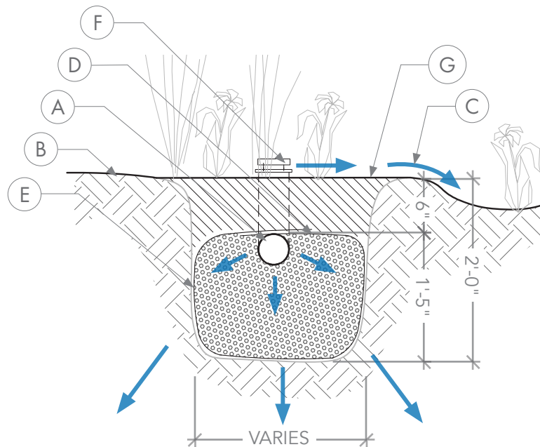
Cross section Through Pumice Wick
