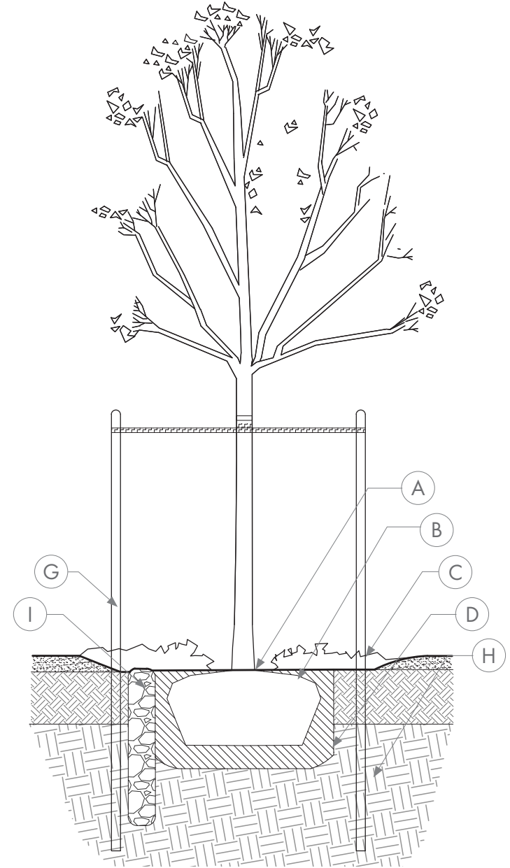
Tree planting diagram
