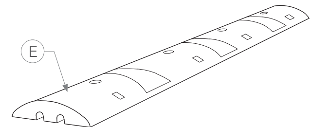
Perspective Detail Speed Bump Deflector
