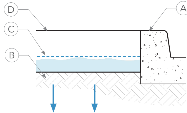
Detail Section of Concrete Curb Basin Border
