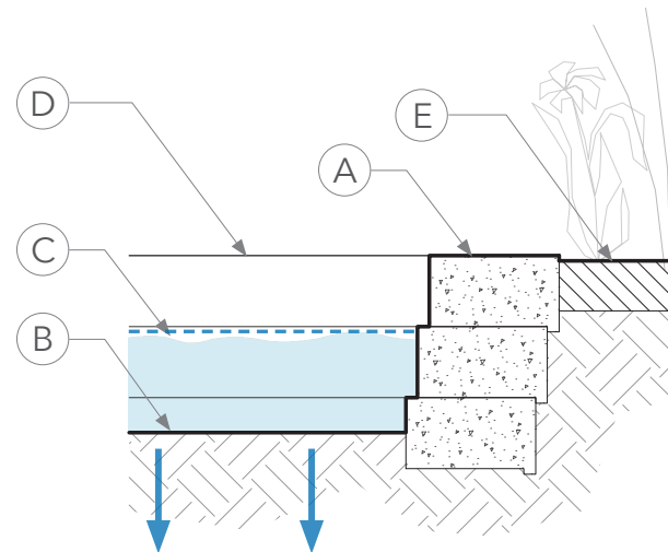
Detail Section of Concrete Block Basin Border
