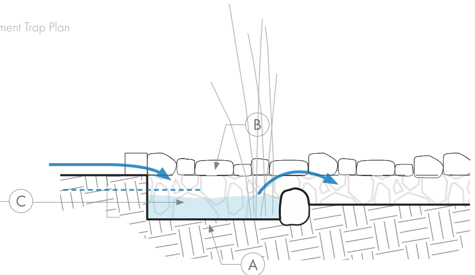
Sediment Trap Section at Parking Space Retrofit
