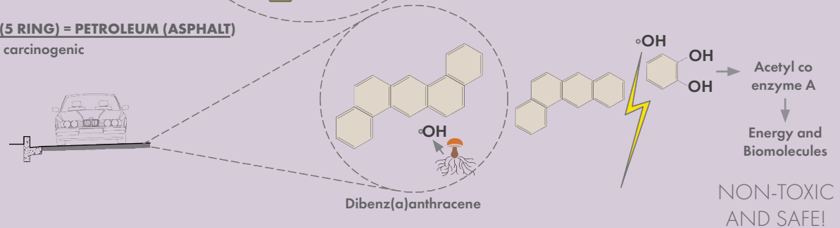
Diagram demonstrating fungal decomposition at a molecular level.
