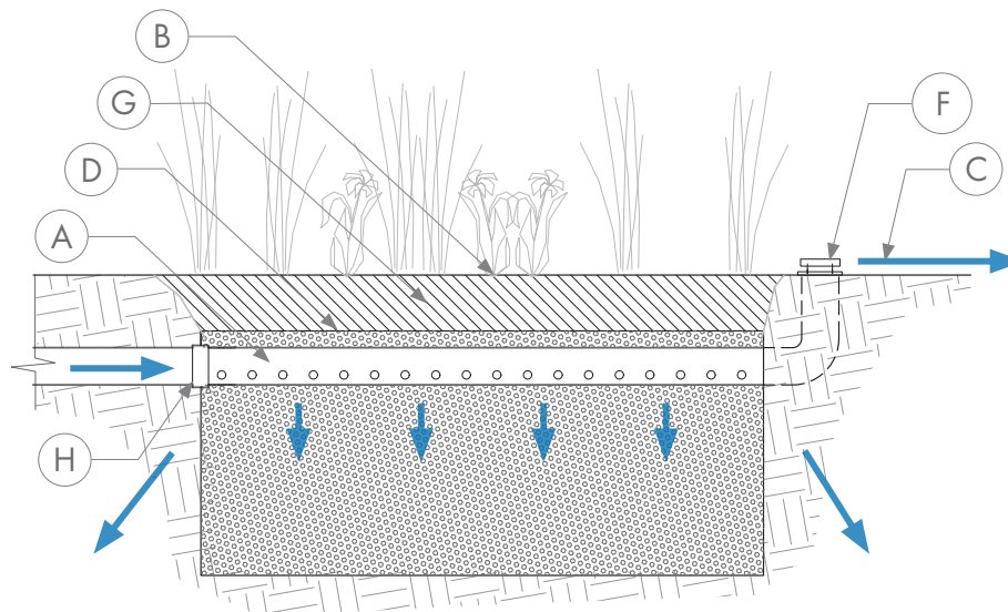
Cross section Through Pumice Wick
