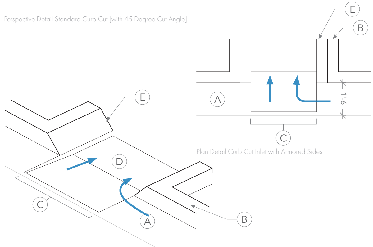
Perspective Detail Curb Cut Inlet with Armored Sides
