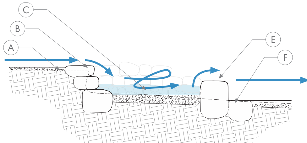
Rural Zuni Bowl Section
