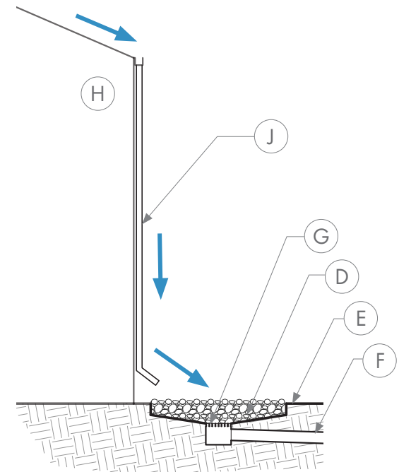
Pitched roof with downspout to catchbasin.
