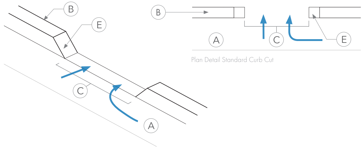
Perspective Detail Standard Curb Cut [with 45 Degree Cut Angle]
