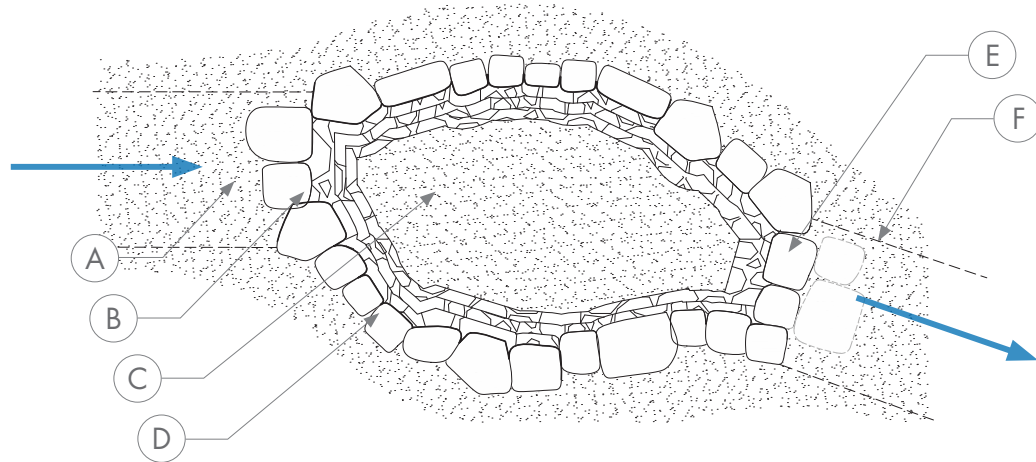
Rural Zuni Bowl Plan
