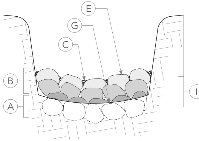
Front Section Detail One Rock Dam (Facing Upstream)
