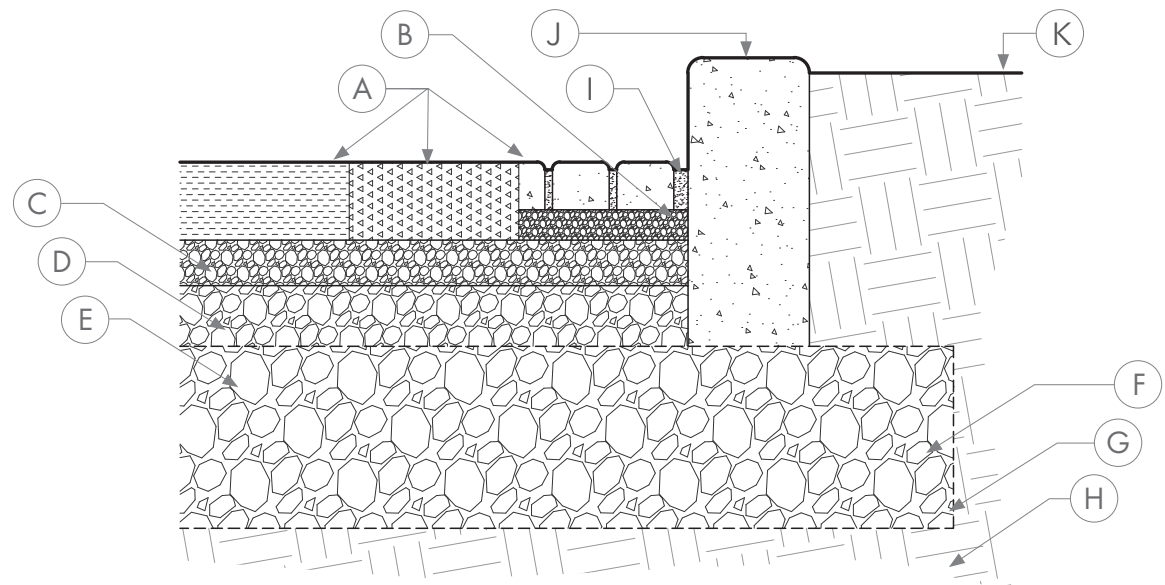
Section through permeable pavement types and underlying substrates
