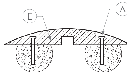
Section Detail Speed Bump Deflector
