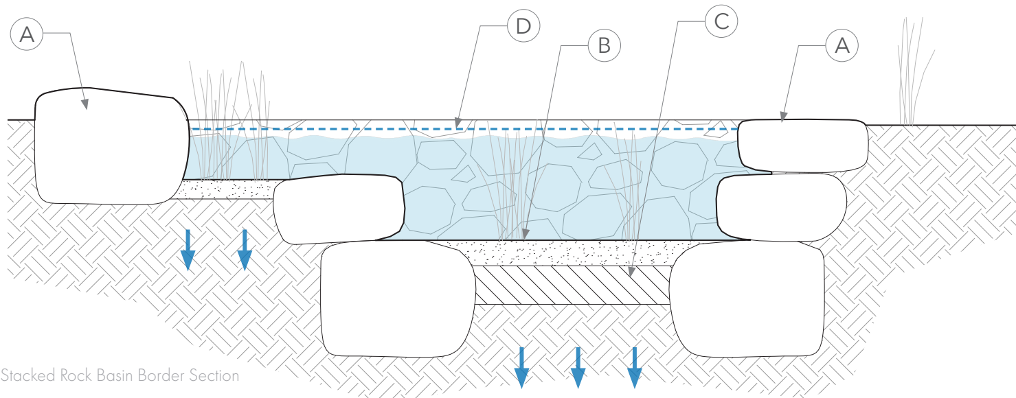
Basin border constructed with Stacked Rock.
