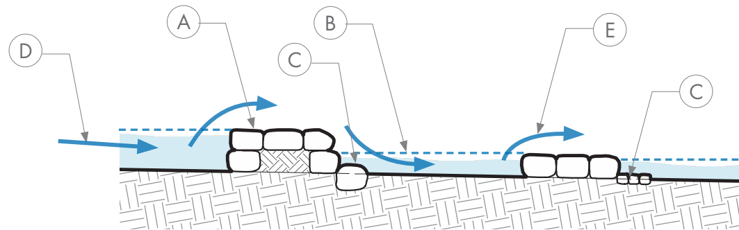
Stone Weir Section
