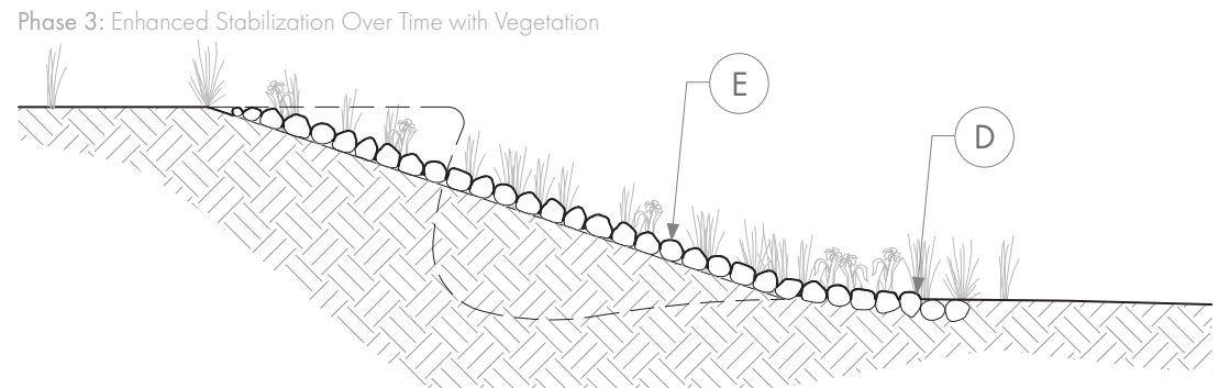
Section Detail Rock Rundown Phasing Over Time - Vegetal Growth
