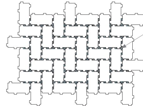
Plan detail of PICPs assembled in interlocking group
