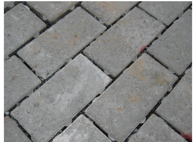
Permeable Interlocking Concrete Pavers (PICP) (Image Credit: Homeguide.com) In ideal style for Southwestern regions. Staggered ridges in between gaps prevent shifting that may block openings. Wider [than standard] gaps increase filtration potential and mitigate sediment build up in arid climates.
