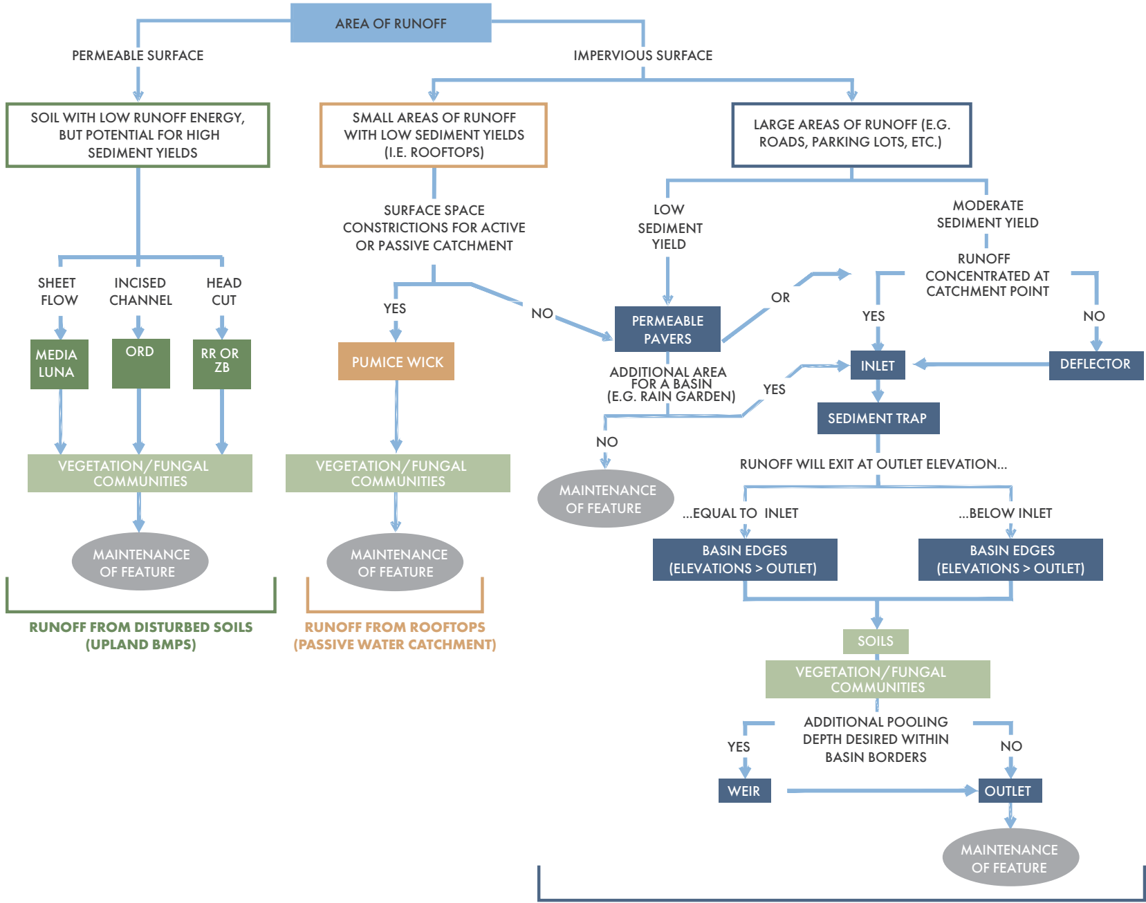
Figure 3. A compilation of components, ordered from upslope to downslope, that can help with GSI and other stormwater management design, installation, and decision making.
