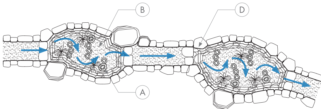
Plan Detail of Myco-sponges used in a series to induce meandering of stormwater in Urban Zuni Bowl rain garden
